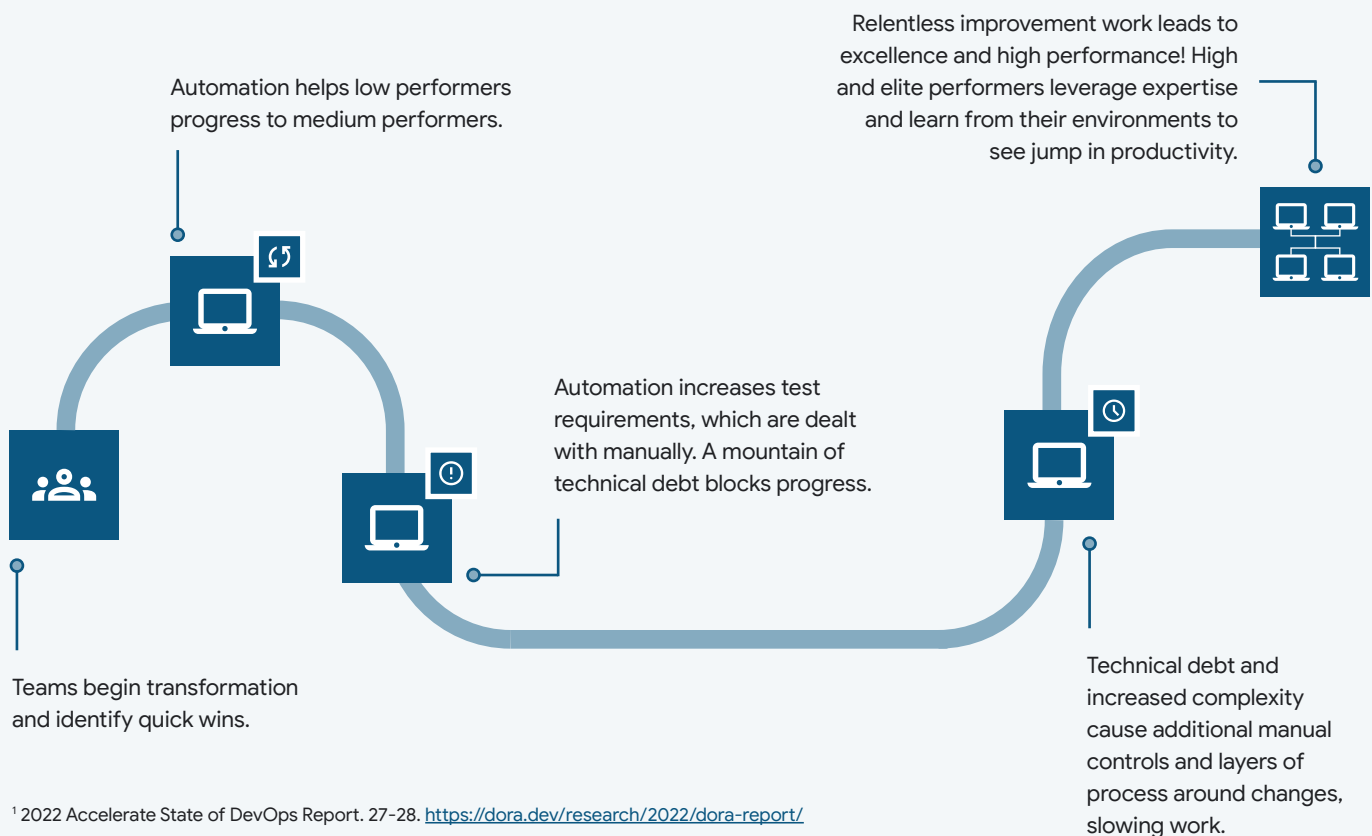
Figure 1: 2018 hypothetical J-curve
